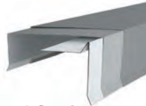
Sloped Coping Continuous Cleat Splice Plate Cover Cap
